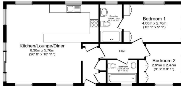
Total floor area 69.1 sq.m. (744 sq.ft.) approx
