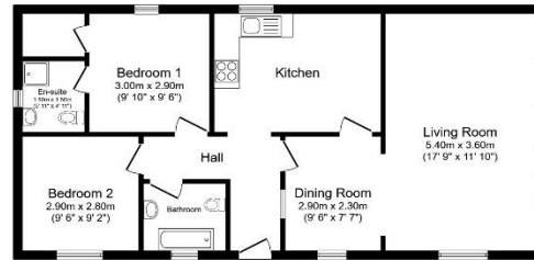
Total floor area 73.8 m 2 (794 sq. ft.) approx
